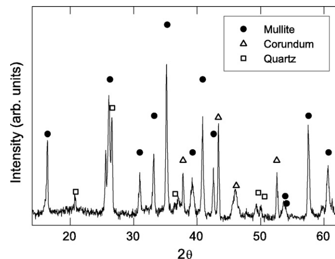
Fig. 8. X-ray diffraction pattern of a coating obtained by reactive plasma spraying of \text{Al}_2\text{O}_3 - \text{SiO}_2 granules.
