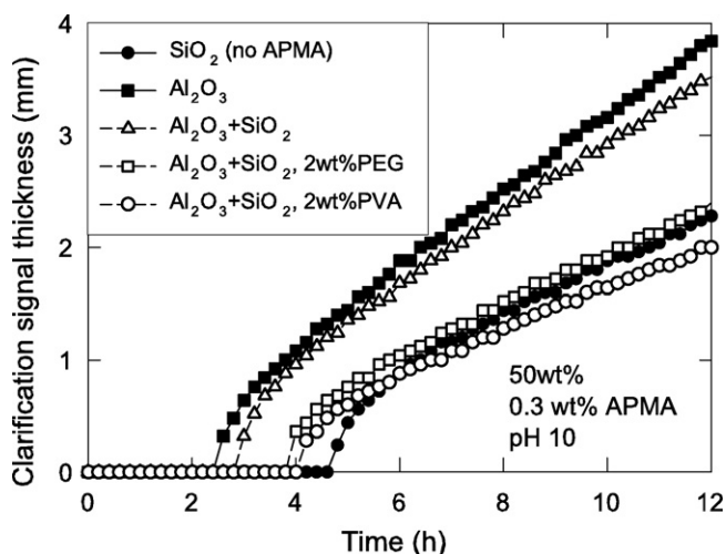
Fig. 3. Sedimentation of various 50 wt% suspensions (pH 10).
