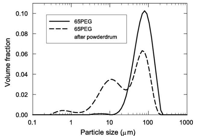
Fig. 6. Granulometric distribution of the PEG65 powder before (plain line) and after (dashed line) the powder-drum experiment.
