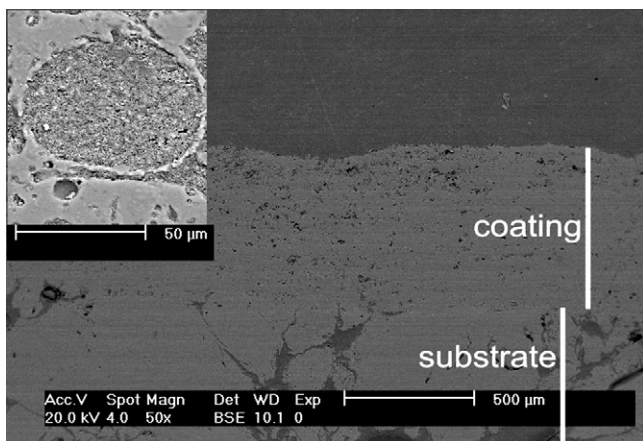
Fig. 7. SEM micrograph of a cross-section through the coating prepared by reactive plasma spray of the 65PEG powder. Inset: Zoom of an unmelted granule.
